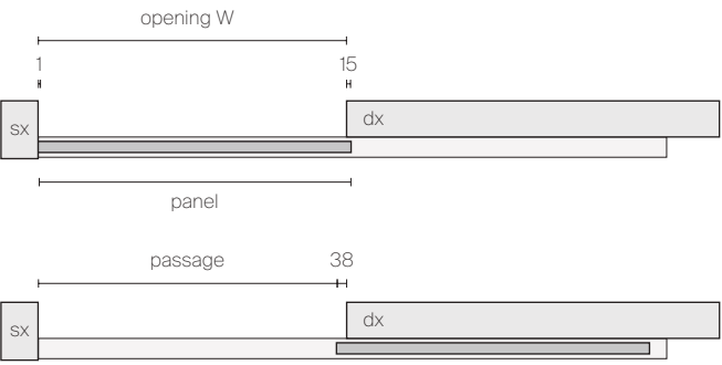
SINGLE SLIDING PANEL COMPOSITION SINGLE RAIL OUT OF THE OPENING
