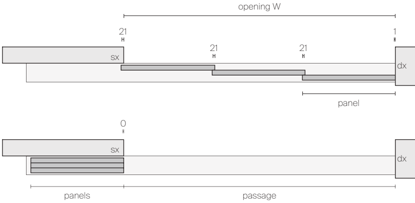
3 SLIDING PANELS COMPOSITION 3 WAYS RAIL OUT OF THE OPENING WITH FLOOR GUIDE PIN AND FLUSH WITH OPEN PANELS
