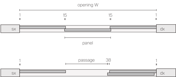
3 SLIDING PANELS COMPOSITION DOUBLE RAIL IN THE OPENING
