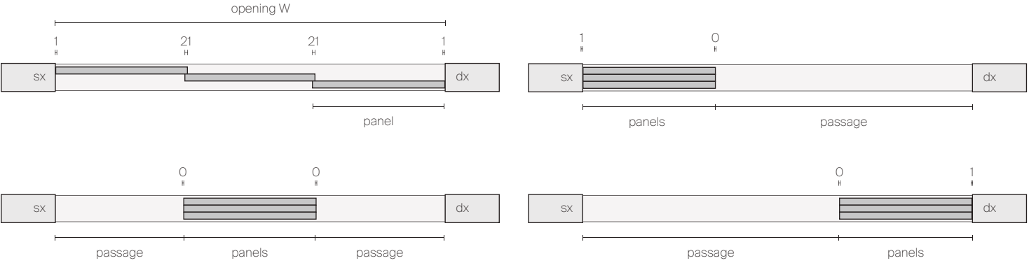
3 SLIDING PANELS COMPOSITION 3 WAYS RAIL IN THE OPENING WITHOUT FLOOR GUIDE PIN AND FLUSH WITH OPEN PANELS
