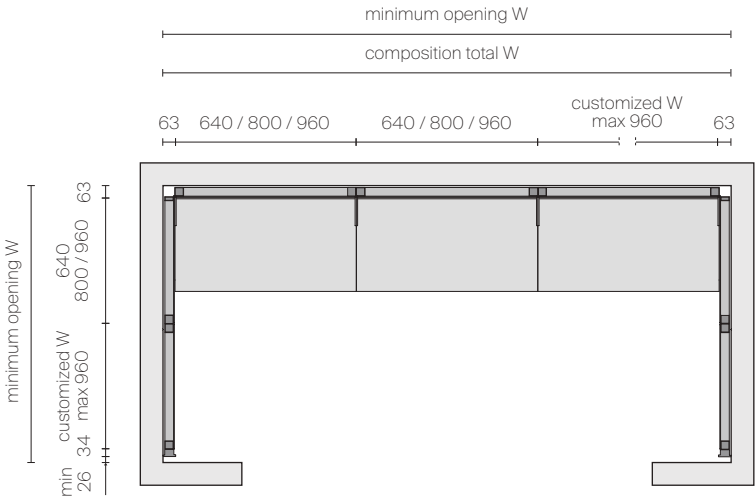
LINEAR COMPOSITION IN NICHE WITH CORNER PANELS WITH TAILORED WIDTH FOR CLADDING USE
