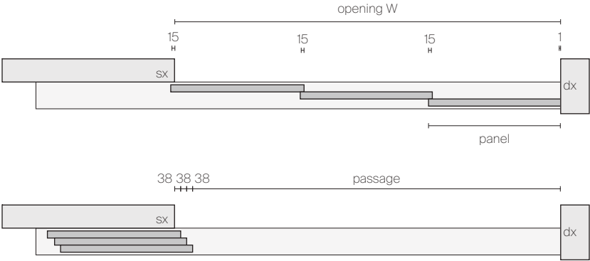
3 SLIDING PANELS COMPOSITION 3 WAYS RAIL OUT OF THE OPENING
