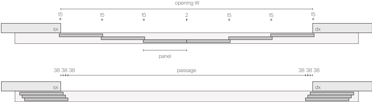
6 SLIDING PANELS COMPOSITION 3 WAYS RAIL OUT OF THE OPENING
