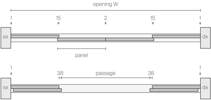
4 SLIDING PANELS COMPOSITION DOUBLE RAIL IN THE OPENING
