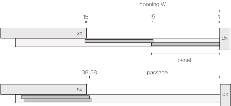
2 SLIDING PANELS COMPOSITION DOUBLE RAIL IN THE OPENING
