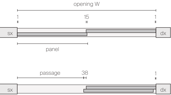
2 SLIDING PANELS COMPOSITION DOUBLE RAIL IN THE OPENING
