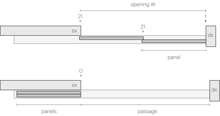
2 SLIDING PANELS COMPOSITION DOUBLE RAIL OUT OF THE OPENING WITH FLOOR GUIDE PIN AND FLUSH WITH OPEN PANELS
