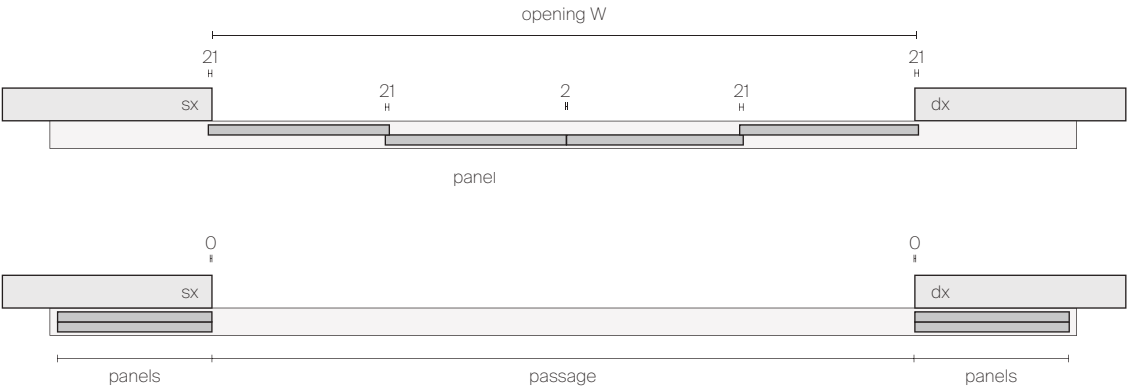
4 SLIDING PANELS COMPOSITION DOUBLE RAIL OUT OF THE OPENING WITH FLOOR GUIDE PIN AND FLUSH WITH OPEN PANELS
