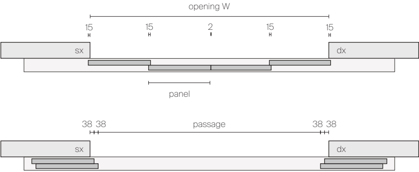
4 SLIDING PANELS COMPOSITION DOUBLE RAIL OUT OF THE OPENING
