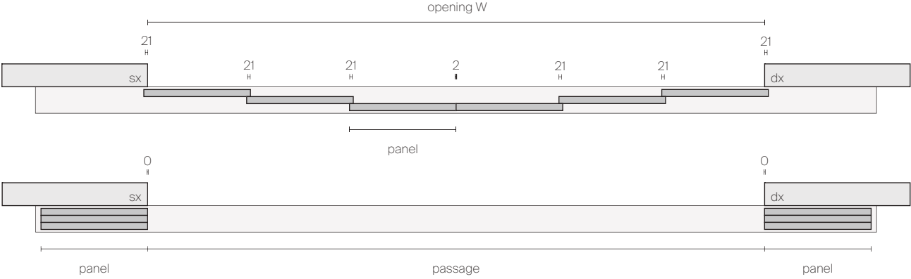
6 SLIDING PANELS COMPOSITION 3 WAYS RAIL OUT OF THE OPENING WITH FLOOR GUIDE PIN AND FLUSH WITH OPEN PANELS
