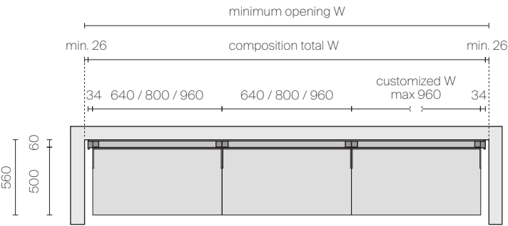
LINEAR COMPOSITION IN NICHE WITH TERMINAL PROFILES
