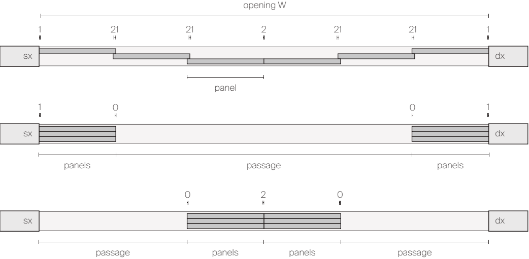
6 SLIDING PANELS COMPOSITION 3 WAYS RAIL IN THE OPENING WITHOUT FLOOR GUIDE PIN AND FLUSH WITH OPEN PANELS
