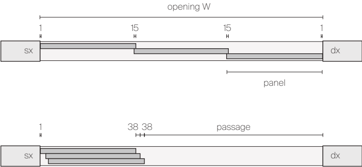
3 SLIDING PANELS COMPOSITION 3 WAYS RAIL IN THE OPENING
