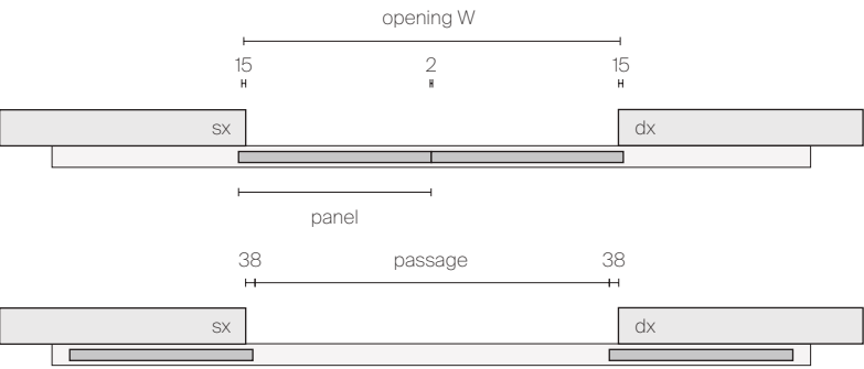
2 SLIDING PANELS COMPOSITION SINGLE RAIL OUT OF THE OPENING
