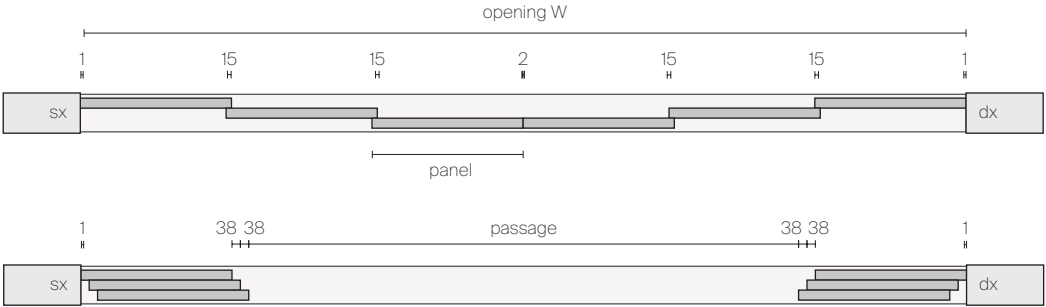
6 SLIDING PANELS COMPOSITION 3 WAYS RAIL IN THE OPENING
