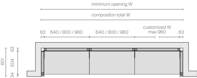
LINEAR COMPOSITION IN NICHE WITH W 504 CORNER PANELS USED AS SIDES
